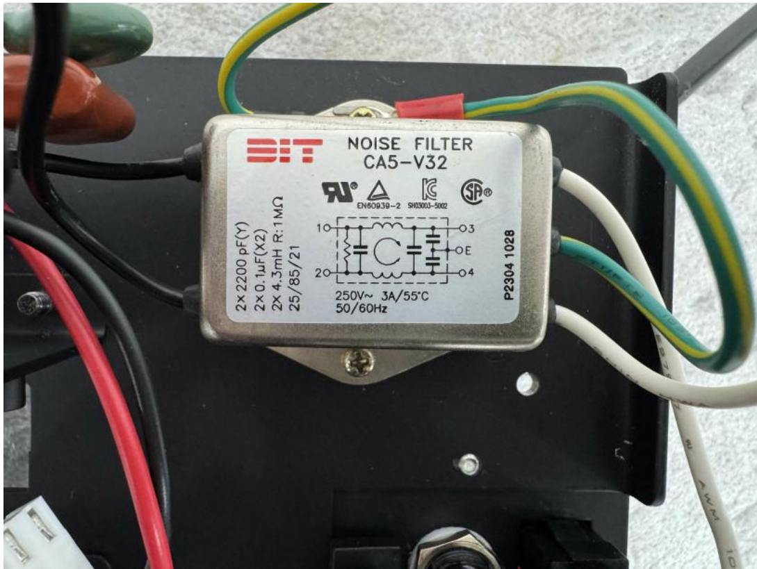
Noise Filter
