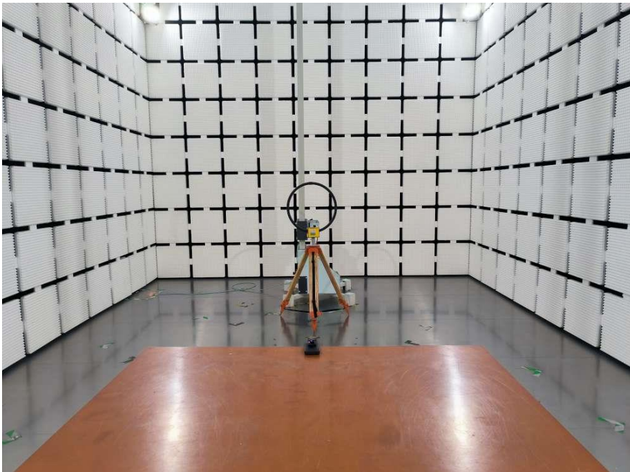
Radiated Emission Test View 8
