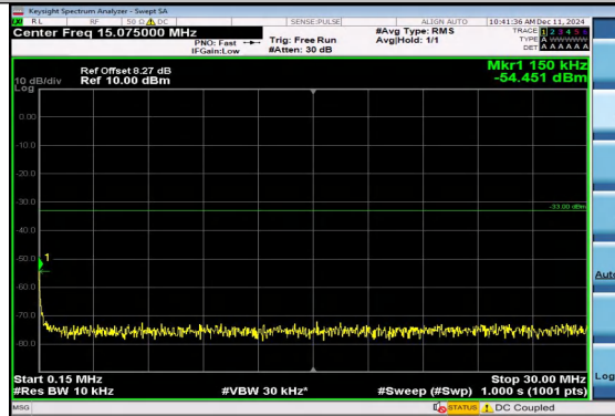
Band2_10MHz_QPSK_18900_1RB#0_0.15~30_0.15~30
