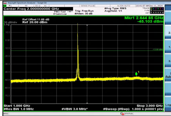
Band2_10MHz_QPSK_18900_1RB#0_1000~3000 _1000~3000
