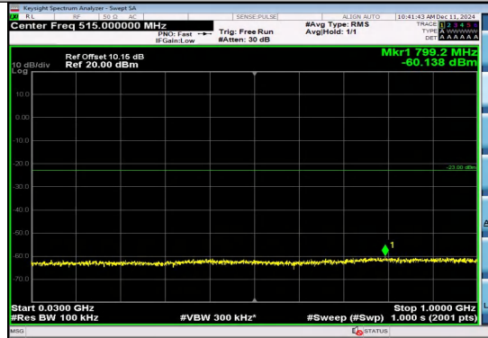
Band2_10MHz_QPSK_18900_1RB#0_30~1000 30~1000
