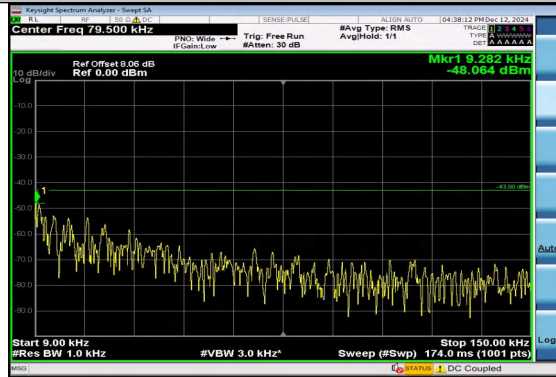
Band2_10MHz_16QAM_18900_1RB#0_0.009~0.15 5_0.009~0.15
