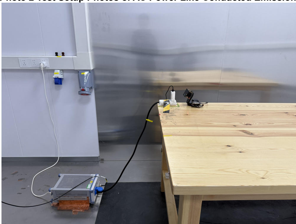
Photo 2 Test Setup Photos of AC Power Line Conducted Emissions
