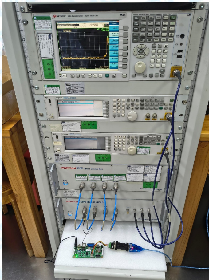
Photo of Setup for Conducted Measurement
