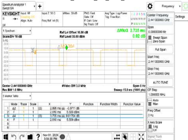
Dwell Time_8DPSK_3M_DH5_2441MHz
