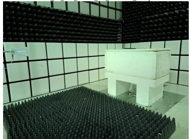
Part 15 407 WLAN 5G Radiated Setup
