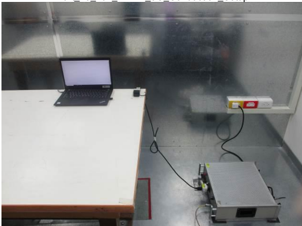
Part_15_407_WLAN_5G_Conduction_Setup
