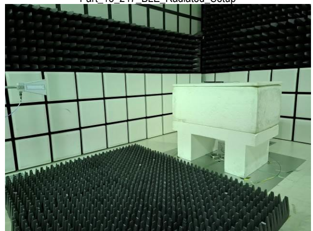
Part_15_247_BLE_Radiated_Setup
