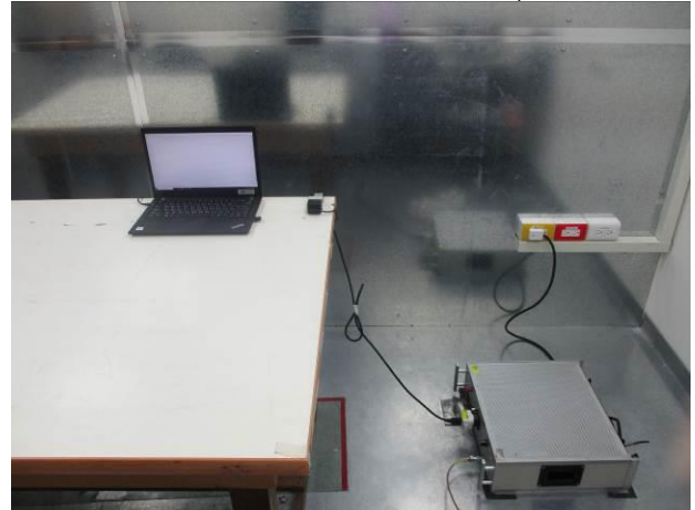
Part_15_247_BT_Conduction_Setup
