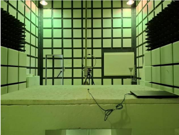
Part_15_247_BT_Radiated_Setup
