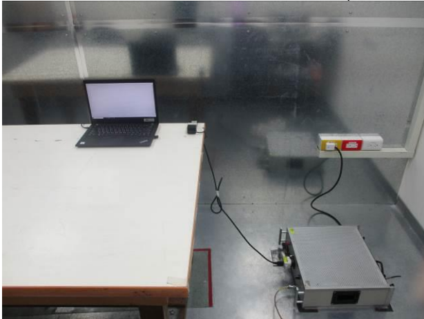
Part_15_247_WLAN_2.4G_Conduction_Setup
