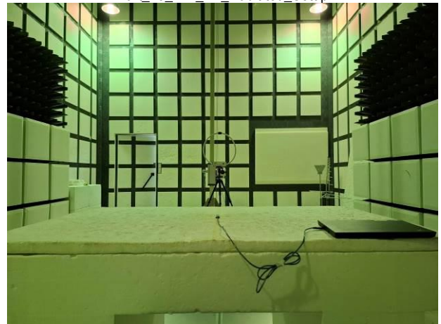
Part_15_247_BT_Radiated_Setup
