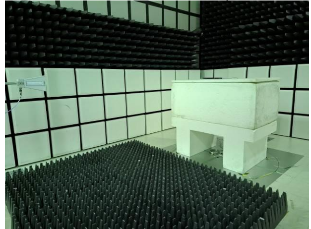
Part_15_247_BT_Radiated_Setup
