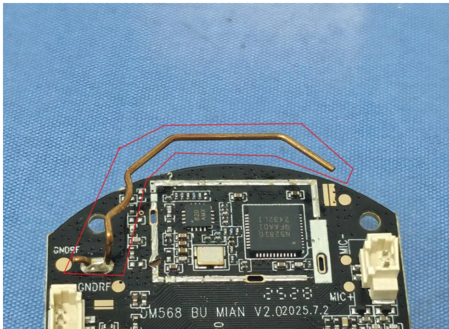
2.4G SRD Antenna
