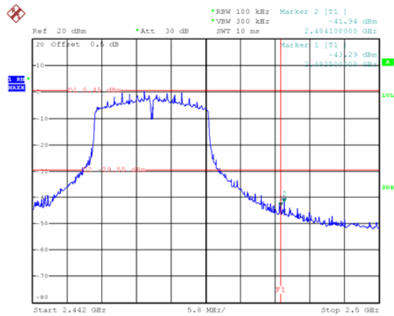
TX 11ax HE20: Band edge-right side
