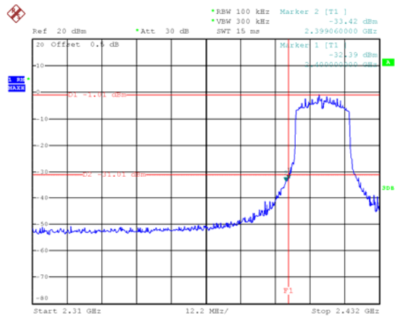
TX 11ax HE20: Band edge-left side
