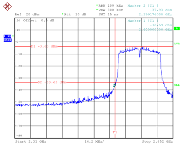
TX 11ax HE40: Band edge-left side
