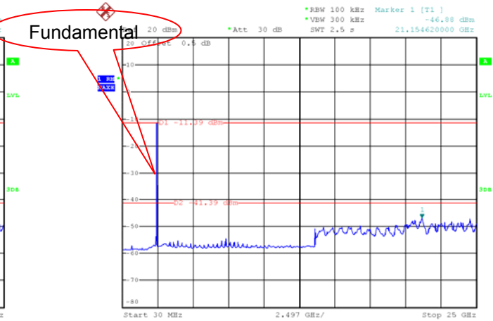
Mode: TX 11 ax HE20 channel 6
