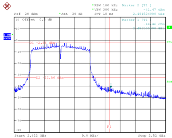
TX 11ax HE40: Band edge-right side
