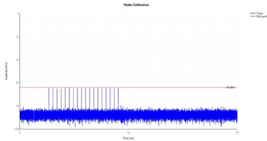
Radar Signal 5270
