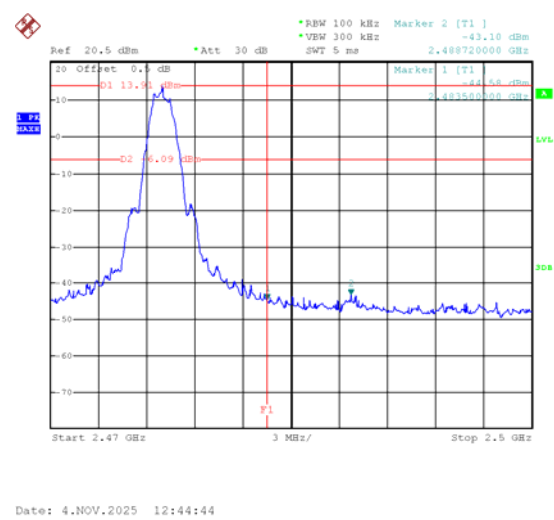
Transmitting Band edge-right side
