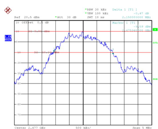
High Channel
