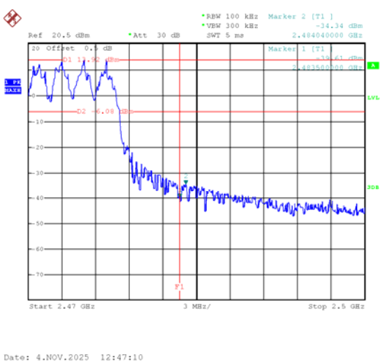
Hopping Band edge-right side
