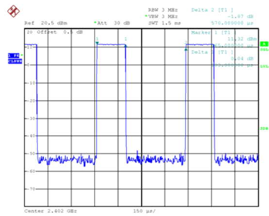
Low Channel
