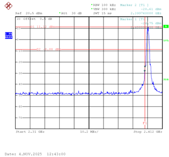
Transmitting Band edge-left side
