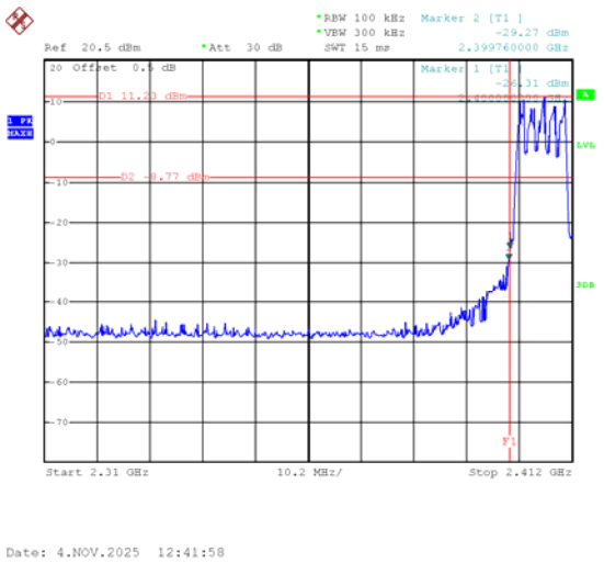
Hopping Band edge-left side
