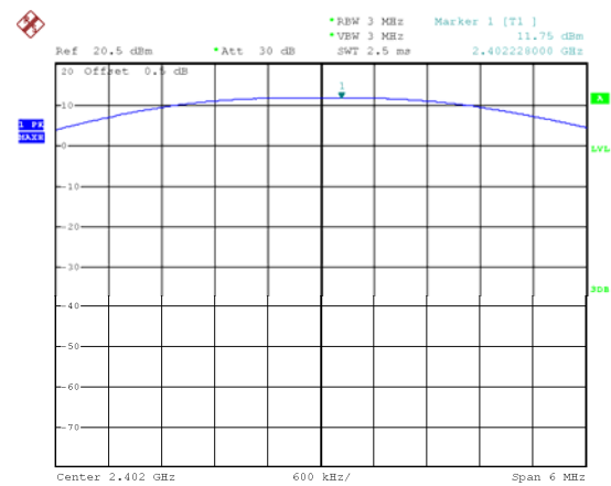
Low Channel
