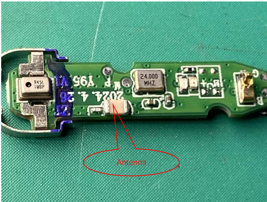
Photo 20 Appearance of PCB---R
