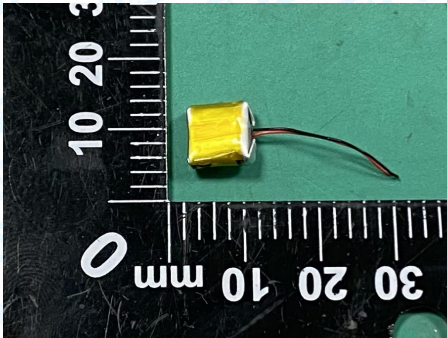
Photo 16 Internal of Battery---R
