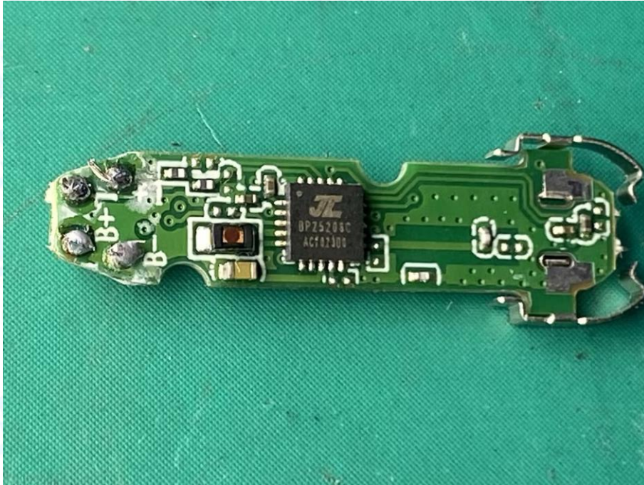
Photo 27 Appearance of PCB---L
