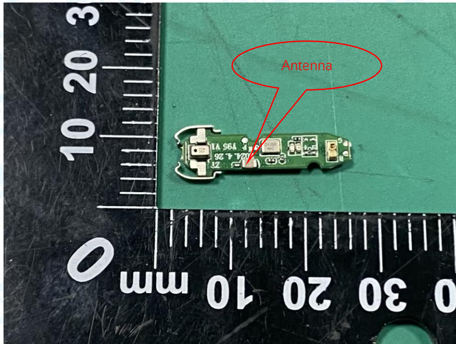
Photo 26 Appearance of PCB---L
