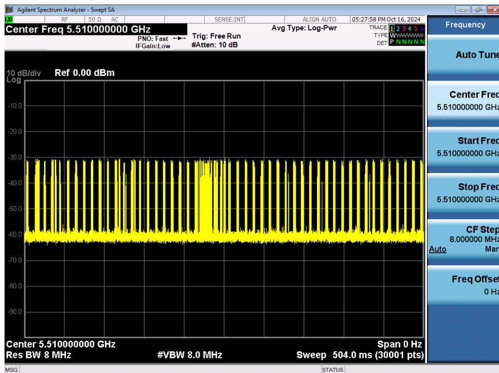
Channel Loading Plot - 802.11n40-5510MHz
