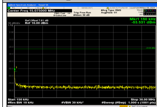
Band5_10MHz_16QAM_20450_1RB#0_0.15~30 0.15~30
