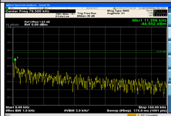
Band5_10MHz_16QAM_20450_1RB#0_0.009~0.15 0.009~0.15
