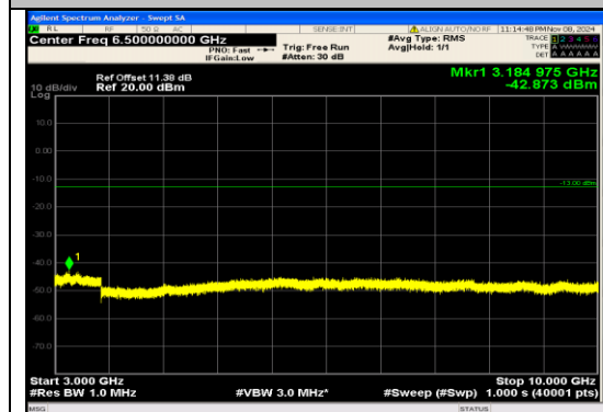
Band5_10MHz_QPSK_20600_50RB#0_3000~10000 3000~10000
