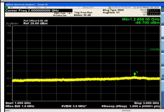
Band5_10MHz_QPSK_20600_50RB#0_1000~3000_1000~3000
