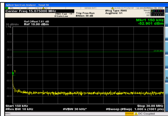
Band5_10MHz_QPSK_20600_50RB#0_0.15~30 _0.15~30
