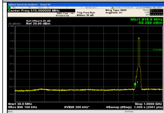
Band5_10MHz_QPSK_20600_50RB#0_30~1000 _30~1000
