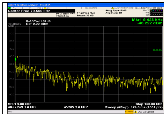
Band5_10MHz_QPSK_20600_50RB#0_0.009~0.15_0.009~0.15
