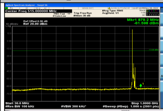
Band5_10MHz_16QAM_20450_1RB#0_30~100 0 30~1000
