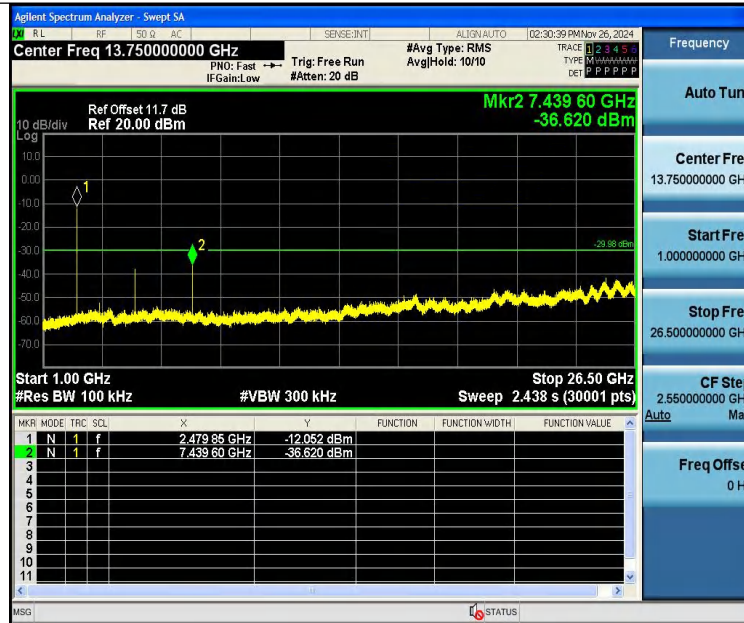
BLE_1M-Ant1-2480-1000~26500-PASS
