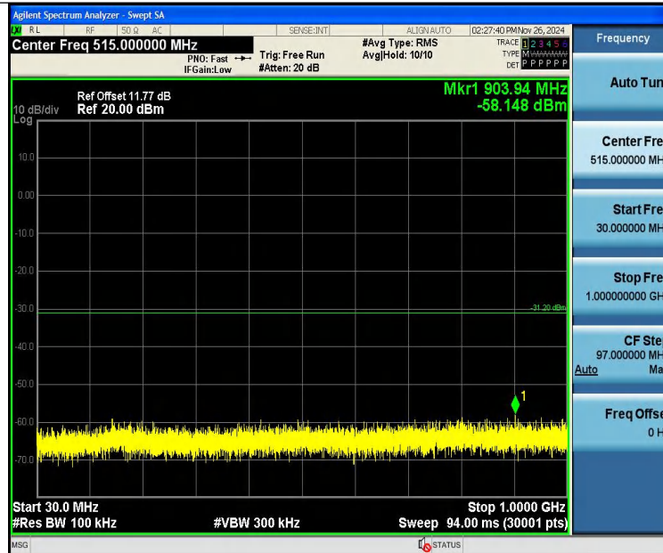
BLE_1M-Ant1-2440-30~1000-PASS
