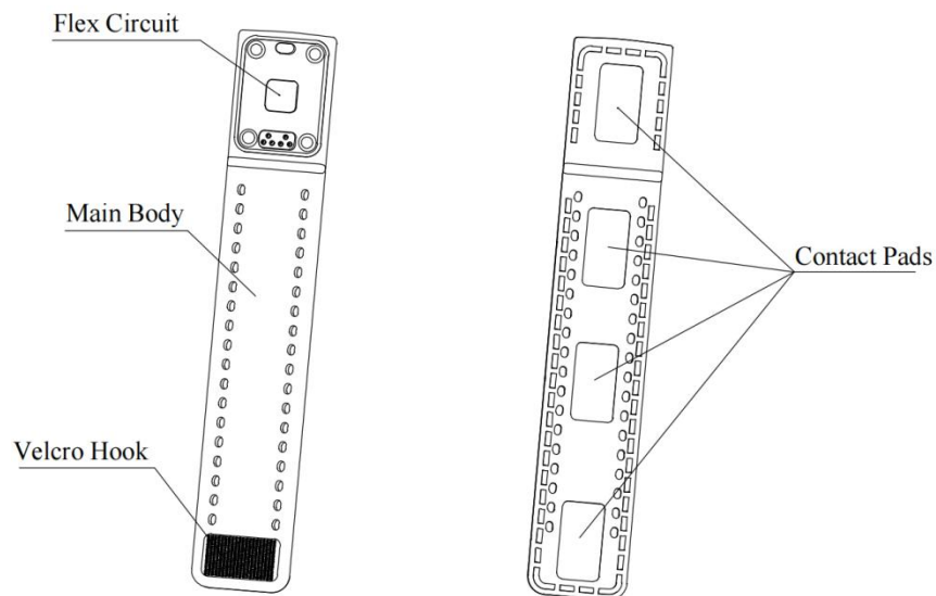
Figure 3. Schematic diagram of the Connector Band
