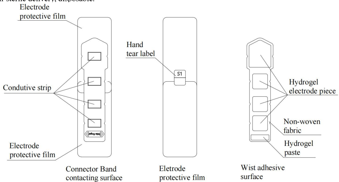
Figure 4 Schematic diagram of Electrode Band
