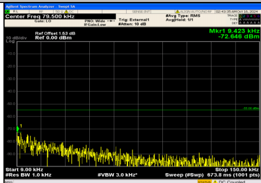
Band38_20MHz_QPSK_37850_100RB#0_0.009 ~0.15_0.009~0.15
