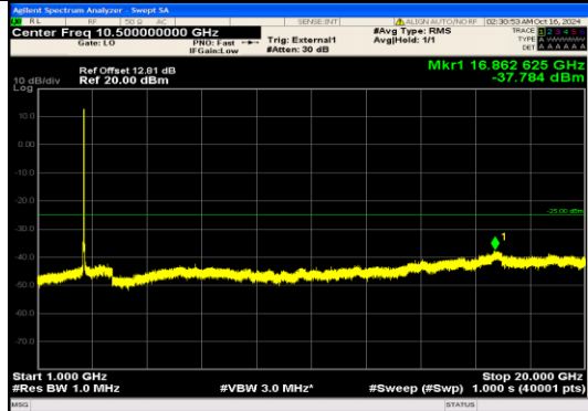
Band38_15MHz_16QAM_38175_75RB#0_1000 ~20000_1000~20000
