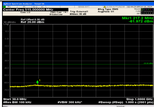
Band38_20MHz_QPSK_37850_100RB#0_30~1 000_30~1000
