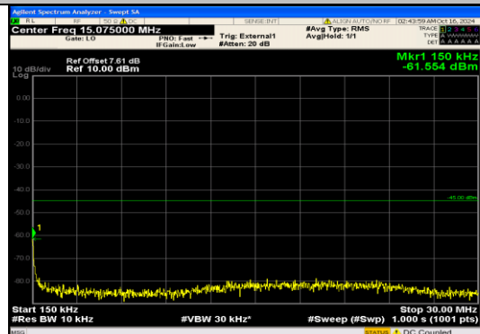
Band38_20MHz_QPSK_37850_100RB#0_0.15~ 30_0.15~30
