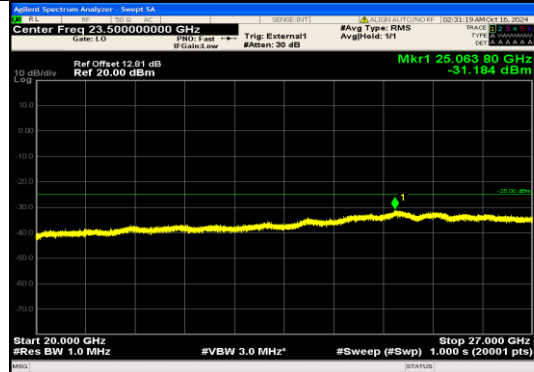
Band38_15MHz_16QAM_38175_75RB#0_2000 0~27000_20000~27000
