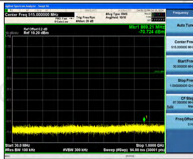
30MHz-1GHz
