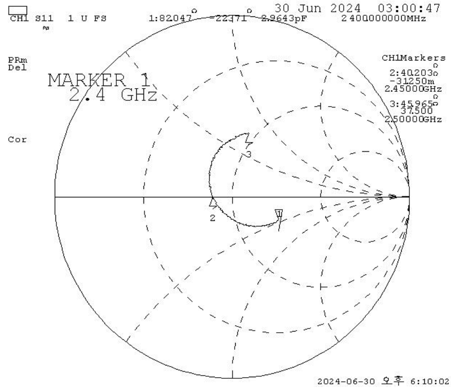
Smith Chart
