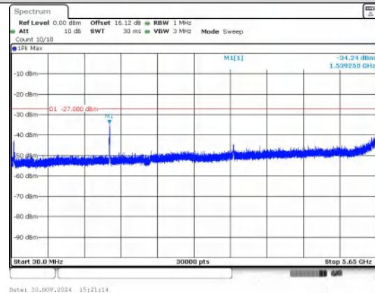
Spurious Emission:30.0~5650 MHz IEEE 802.11n_Channel 149_20MHz_Antenna 0
