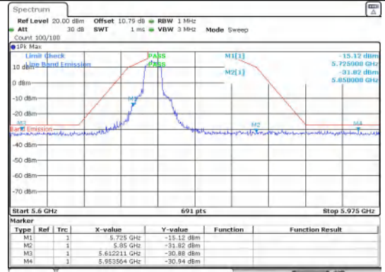
Out Of Band Emission IEEE 802.11n_Channel 149_20MHz_Antenna 1
