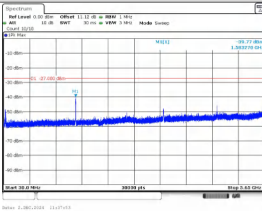
Spurious Emission:30.0~5650 MHz IEEE 802.11a_Channel 157_20MHz_Antenna 1
