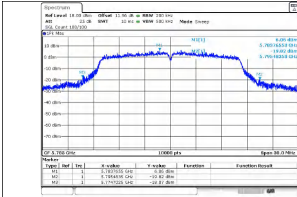
IEEE 802.11a_Channel 157_20MHz_Antenna 0
