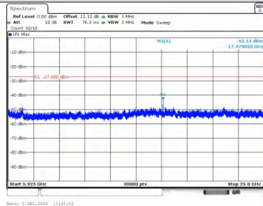
Spurious Emission:5925~25000.0 MHz IEEE 802.11a_Channel 165_20MHz_Antenna 1
