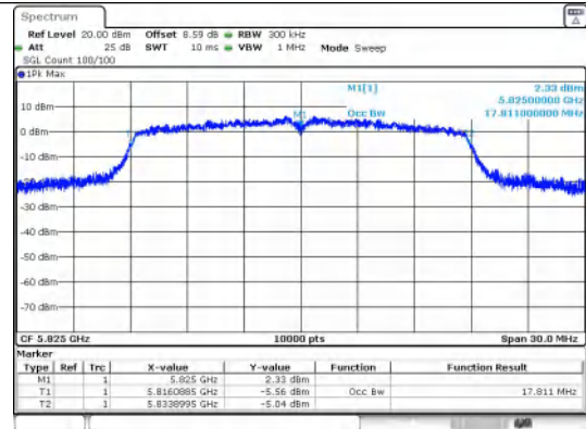
IEEE 802.11ac_Channel 165_20MHz_Antenna 1
