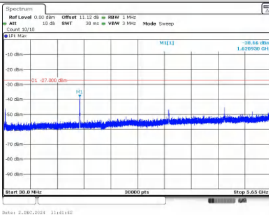
Spurious Emission:30.0~5650 MHz IEEE 802.11a_Channel 165_20MHz_Antenna 1
