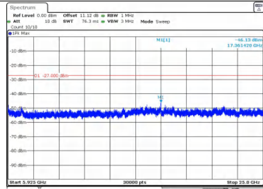
Out Of Band Emission IEEE 802.11n_Channel 157_20MHz_Antenna 1
