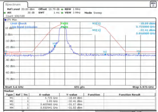
Out Of Band Emission IEEE 802.11ac_Channel 149_20MHz_Antenna 1
