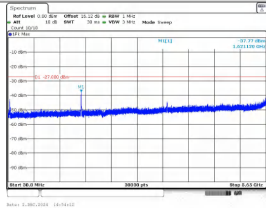
Spurious Emission:30.0~5650 MHz IEEE 802.11a_Channel 165_20MHz_Antenna 0
