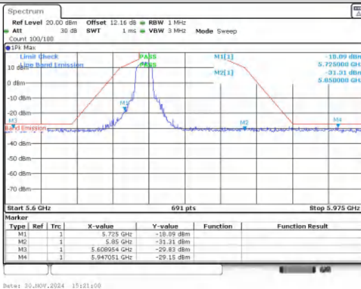
Out Of Band Emission IEEE 802.11n_Channel 149_20MHz_Antenna 0
