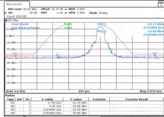
Out Of Band Emission IEEE 802.11ac_Channel 165_20MHz_Antenna 1
