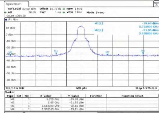
Out Of Band Emission IEEE 802.11a_Channel 157_20MHz_Antenna 1
