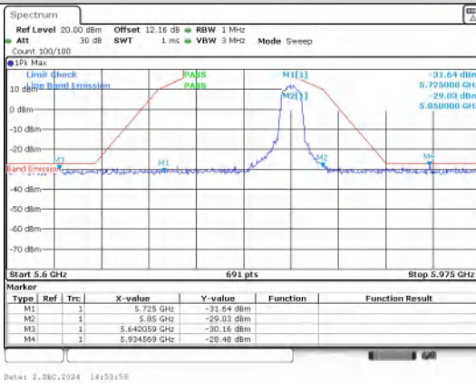
Out Of Band Emission IEEE 802.11a_Channel 165_20MHz_Antenna 0
