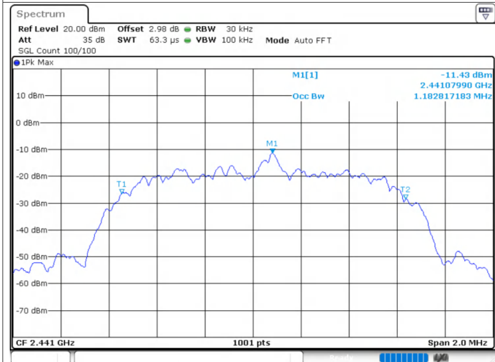
OBW NVNT 2-DH5 2441MHz Ant1
