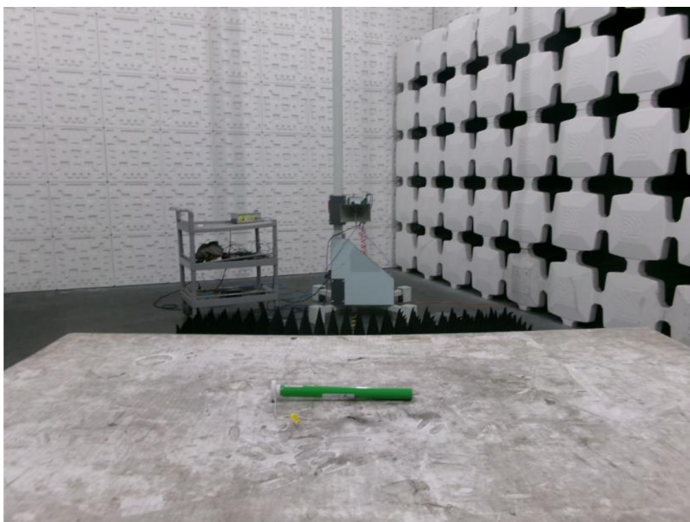
Radiated Setup for Above 1 GHz
