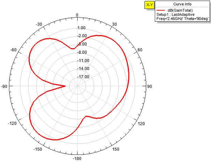
Radiation Pattern 2
