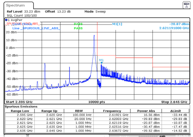
15MHz_High_16QAM_1@74
