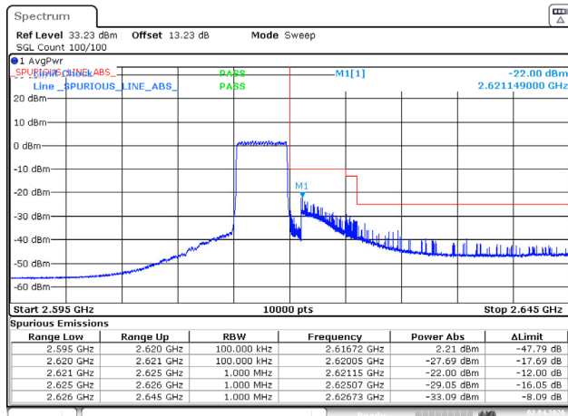
5MHz_High_16QAM_25@0
