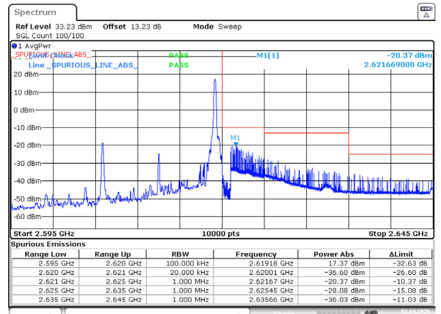
15MHz_High_QPSK_1@74
