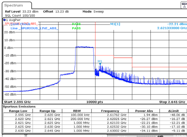
10MHz_High_16QAM_27@23
