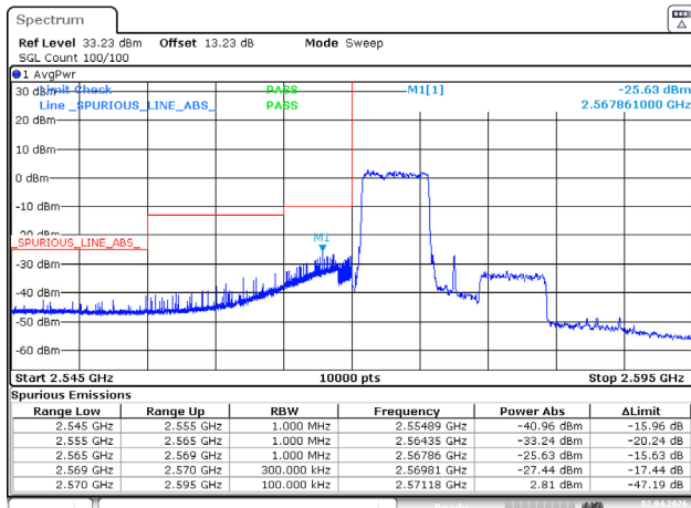
15MHz_Low_16QAM_27@0
