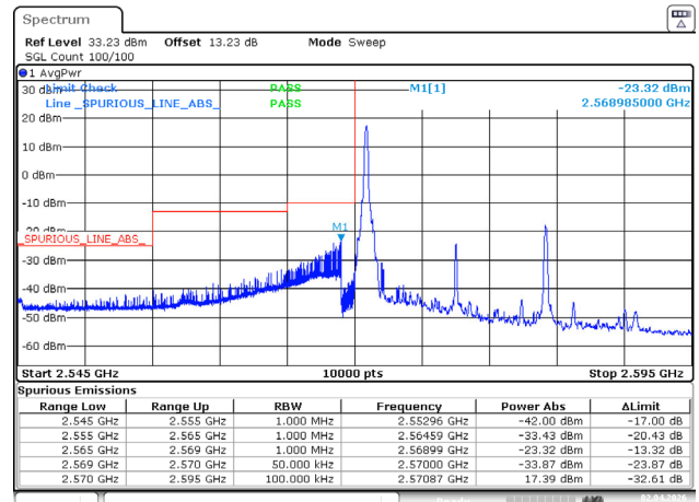
15MHz_Low_QPSK_1@0
