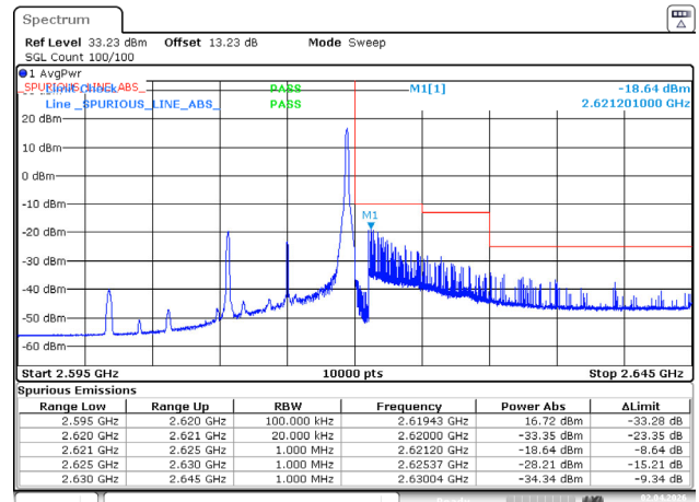
10MHz_High_16QAM_1@49
