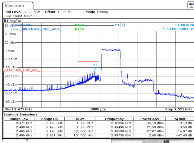
15MHz_Low_16QAM_27@0
