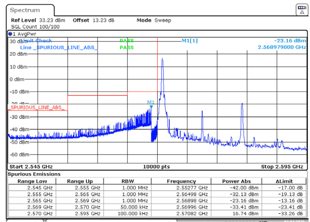
15MHz_Low_16QAM_1@0
