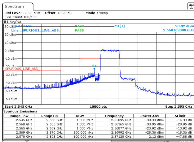
10MHz_Low_16QAM_27@0
