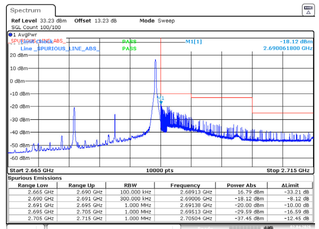
15MHz_High_16QAM_1@74
