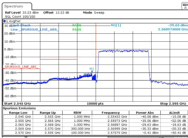
15MHz_Low_QPSK_75@0
