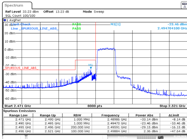
10MHz_Low_16QAM_27@0
