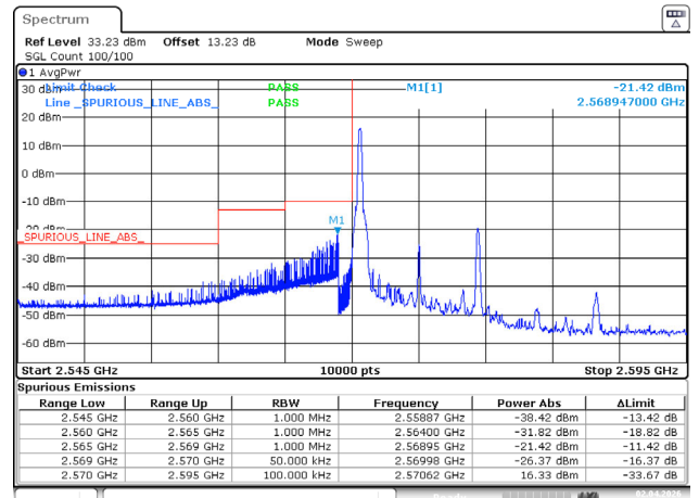
10MHz_Low_16QAM_1@0
