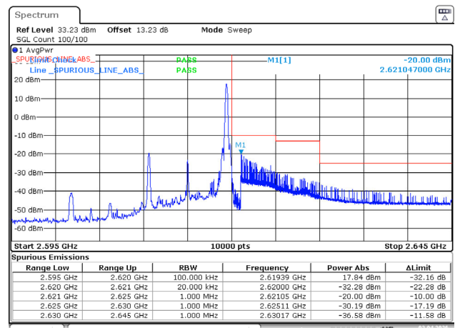
10MHz_High_QPSK_1@49
