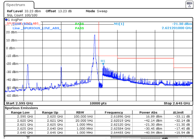
20MHz_High_QPSK_1@99
