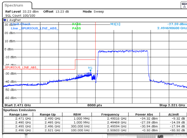
15MHz_Low_QPSK_75@0
