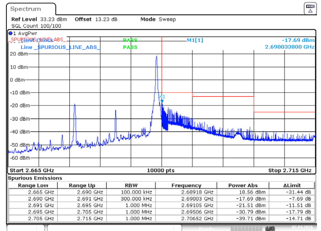
15MHz_High_QPSK_1@74
