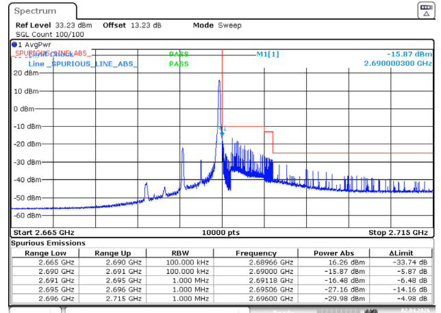
5MHz_High_16QAM_1@24
