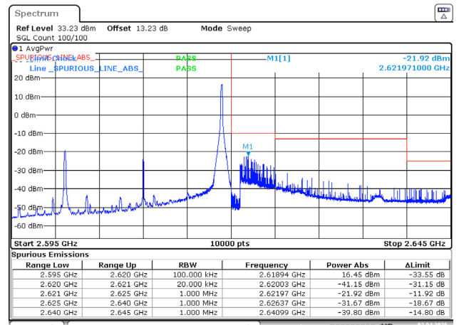
20MHz_High_16QAM_1@99
