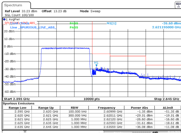
15MHz_High_QPSK_75@0
