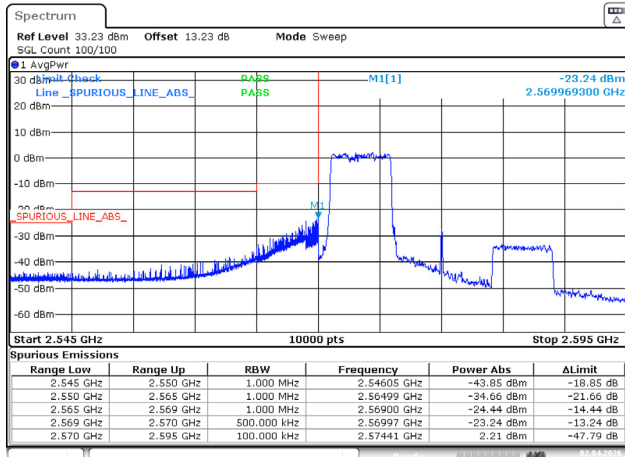
20MHz_Low_16QAM_27@0
