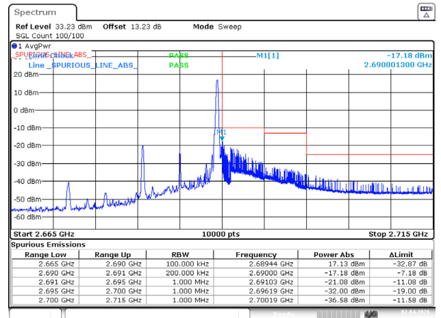
10MHz_High_QPSK_1@49
