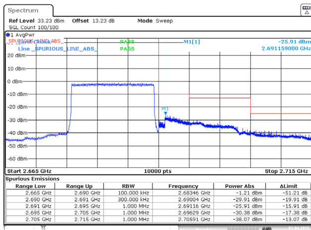
15MHz_High_QPSK_75@0
