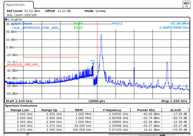
20MHz_Low_16QAM_1@0
