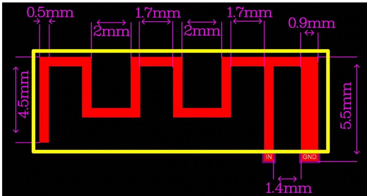
Antenna Photo & Length (mm)
