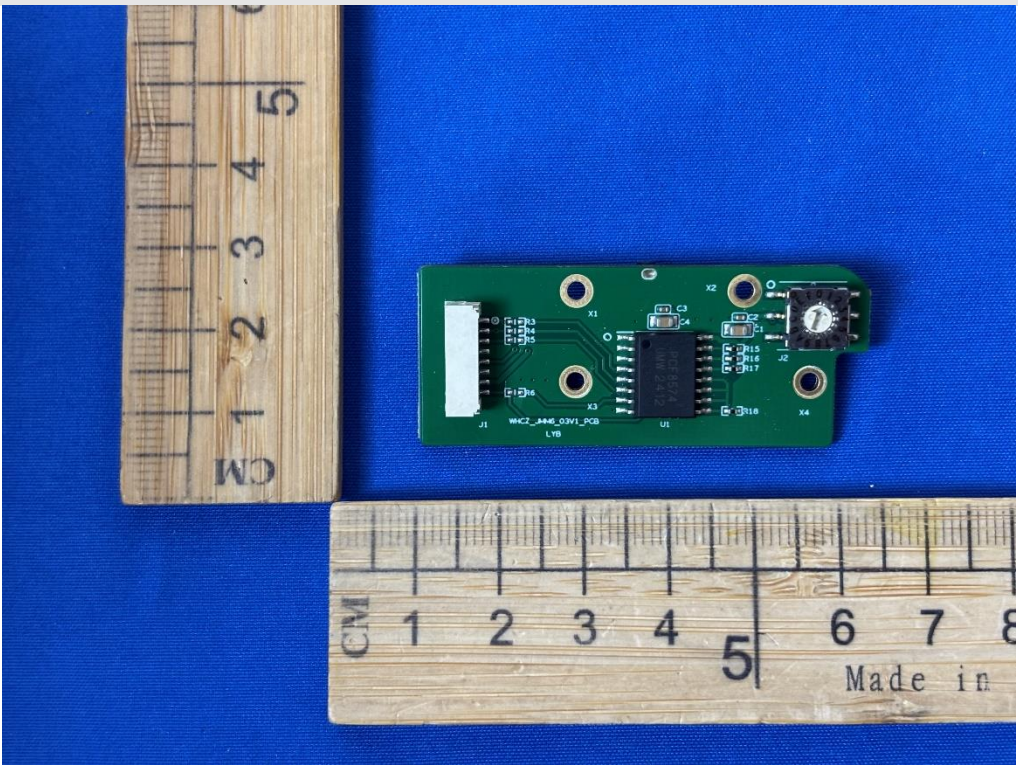
Internal View of EUT-42
