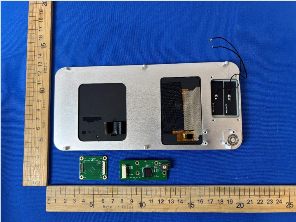
Internal View of EUT-39
