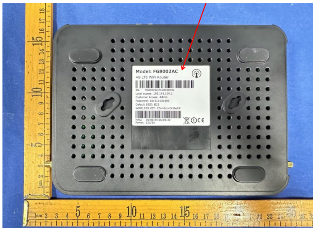
Lable Location
