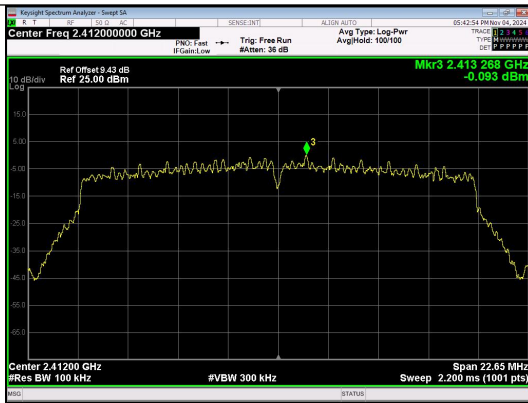
In-Band Reference Level IEEE 802.11n Channel 1 20MHz Antenna 1
