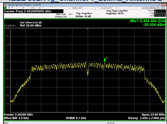
IEEE 802.11g_Channel 11_20MHz_Antenna 2
