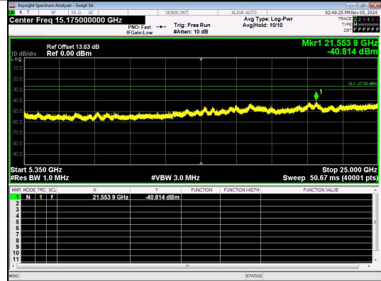
Spurious Emission:5350~25000.0 MHz IEEE 802.11n Channel 36 20MHz Antenna 4
