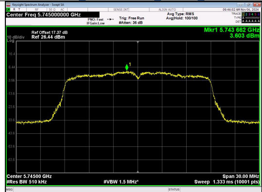
IEEE 802.11n Channel 149 20MHz Antenna 3
