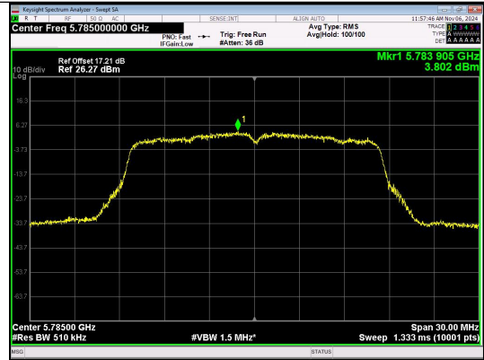
IEEE 802.11a Channel 157 20MHz Antenna 3
