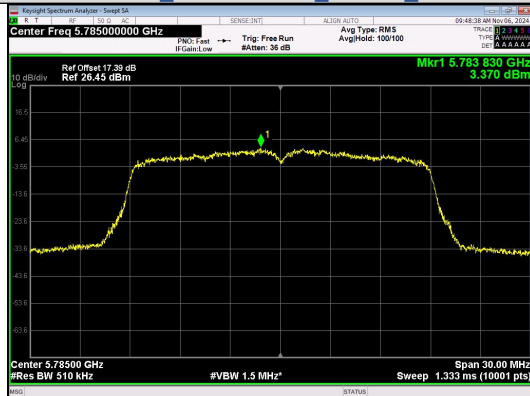
IEEE 802.11n Channel 157 20MHz Antenna 3
