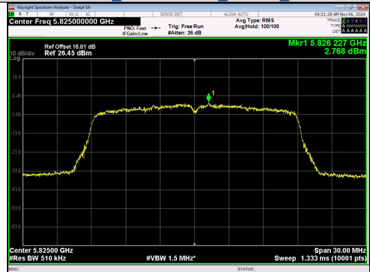
IEEE 802.11n Channel 165 20MHz Antenna 3
