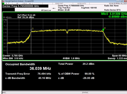
IEEE 802.11ac Channel 159 40MHz Antenna 3
