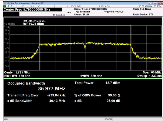
IEEE 802.11n Channel 159 40MHz Antenna 4
