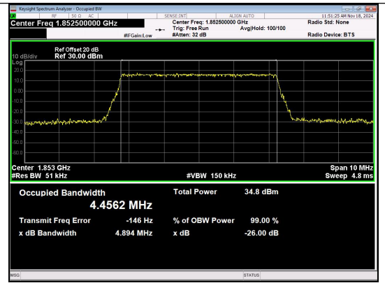
Band 2 5MHz/1852.5/High 16QAM 25@0
