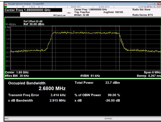
Band 2 3MHz/1880.0/Mid 16QAM 15@0
