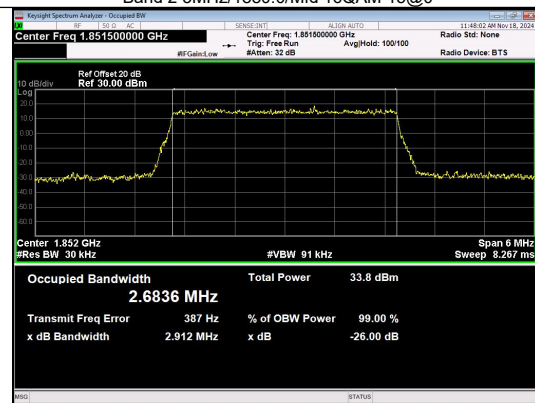
Band 2 3MHz/1851.5/Low 16QAM 15@0
