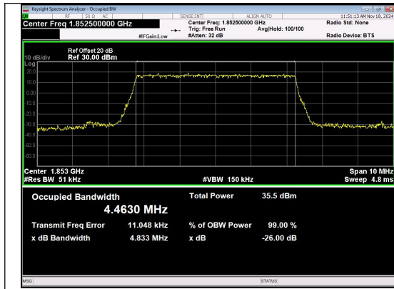
Band 2 5MHz/1852.5/High QPSK 25@0
