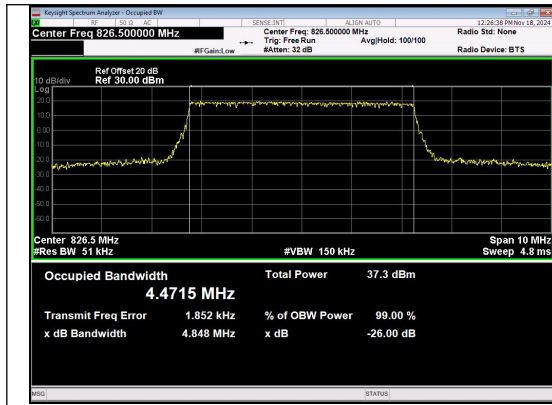
Band 5 5MHz/826.5/High QPSK 25@0
