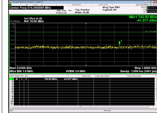
30.0MHz-1000.0MHz Band 2 15MHz/1902.5/High 16QAM 1@0
