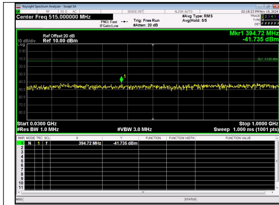
30.0MHz-1000.0MHz Band 2 5MHz/1852.5/Low QPSK 1@0
