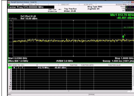
30.0MHz-1000.0MHz Band 2 20MHz/1900.0/High QPSK 1@0
