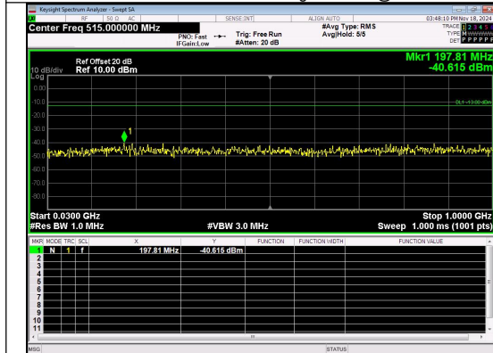
30.0MHz-1000.0MHz Band 2 20MHz/1900.0/High 16QAM 1@0
