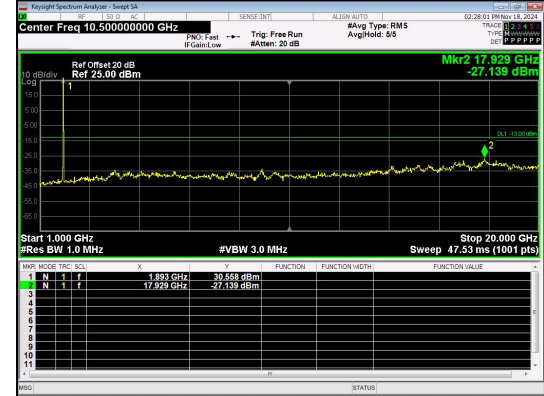
1000.0MHz-20000.0MHz Band 2 15MHz/1902.5/High 16QAM 1@0
