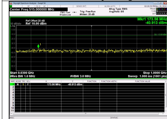
30.0MHz-1000.0MHz Band 2 10MHz/1905.0/High 16QAM 1@0
