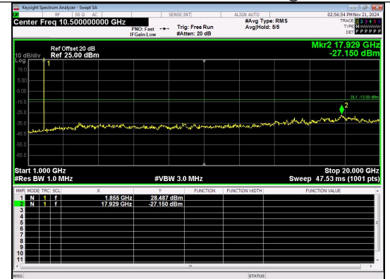
1000.0MHz-20000.0MHz Band 2 10MHz/1855.0/Low QPSK 1@0
