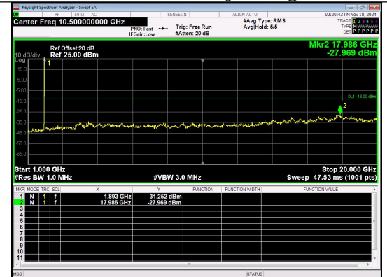
1000.0MHz-20000.0MHz Band 2 10MHz/1905.0/High 16QAM 1@0
