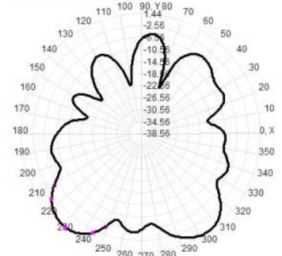
Total(H-XY), Max= 1.44dBi, CirD=23.62
