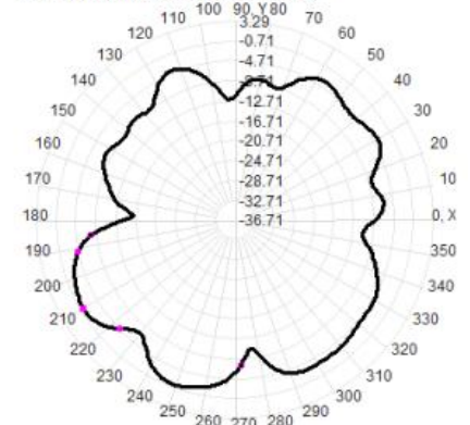
Total(H-XY), Max= -1.54dBi, CirD=14.67
