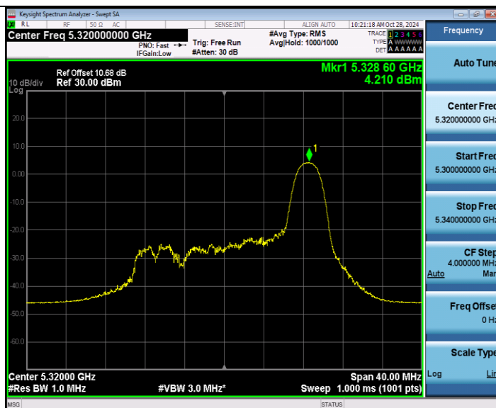
11AX20MIMO Ant W0 5320 52Tone RU40
