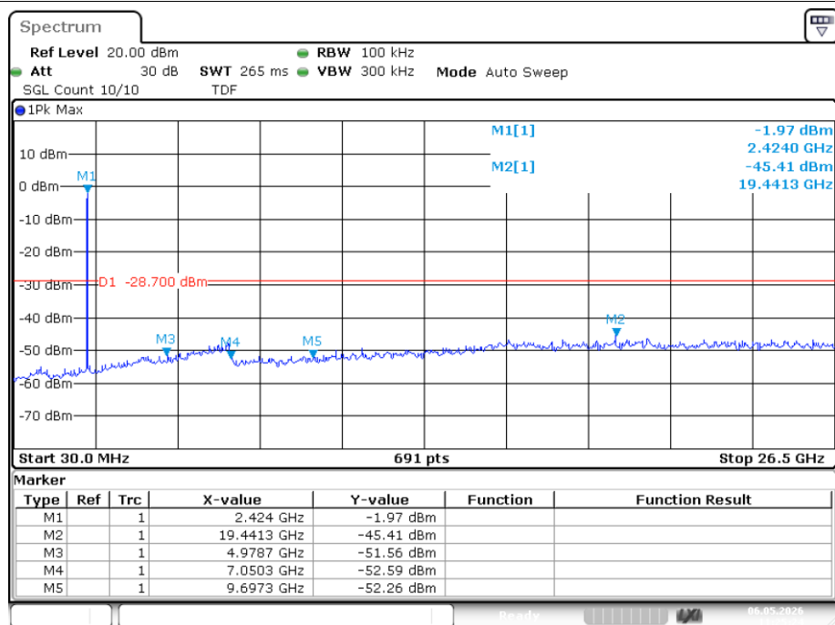
Tx. Spurious NVNT n20 2412MHz Ant2 Ref
