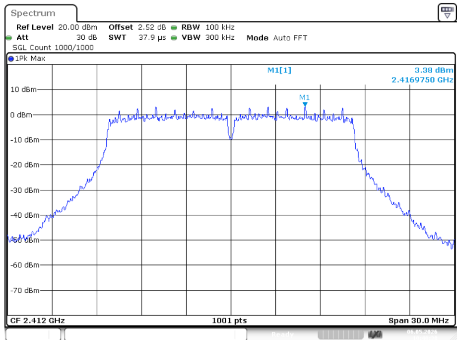
Band Edge NVNT g 2412MHz Ant2 Ref
