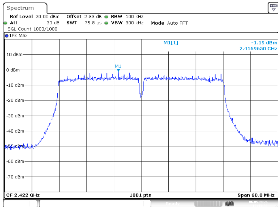
Band Edge NVNT n40 2422MHz Ant2 Ref
