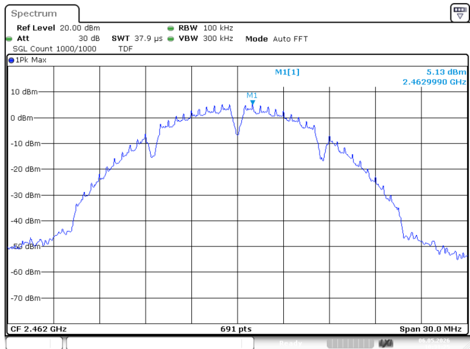
Tx. Spurious NVNT b 2462MHz Ant2 Ref
