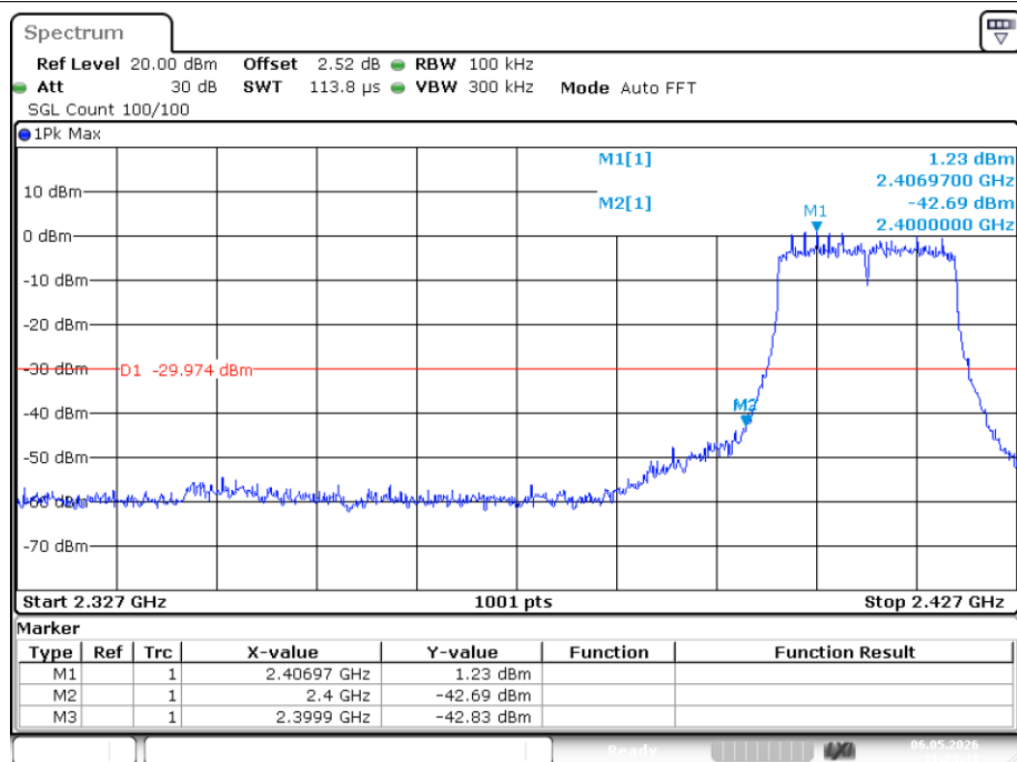
Band Edge NVNT n20 2412MHz Ant2 Ref
