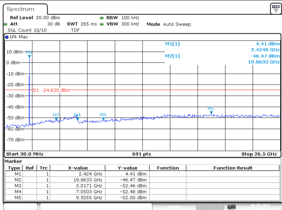
Tx. Spurious NVNT b 2412MHz Ant2 Ref
