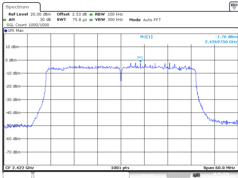
Band Edge NVNT ax40 2422MHz Ant2 Ref
