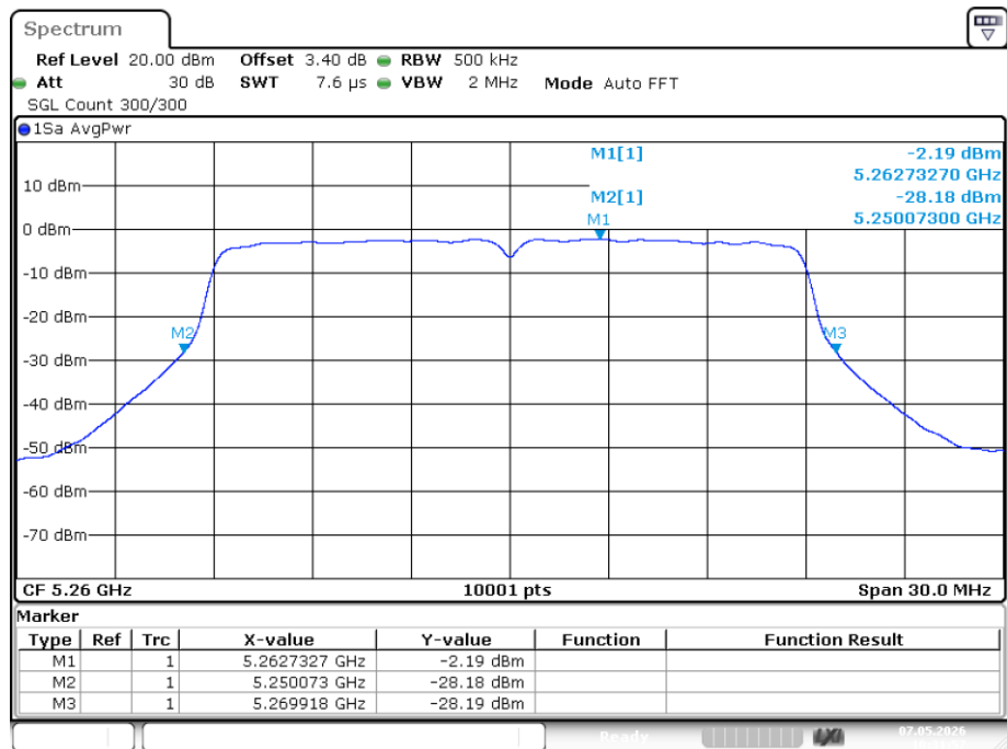
-26dB Bandwidth NVNT ac20 5260MHz Ant1
