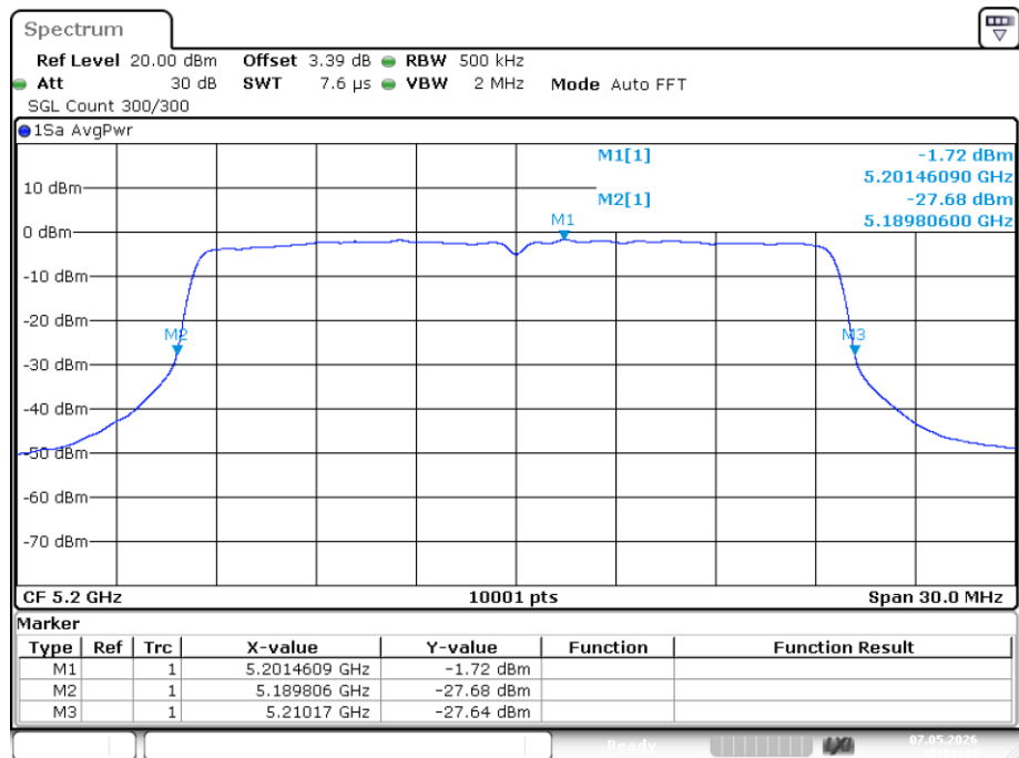
-26dB Bandwidth NVNT ax20 5200MHz Ant1
