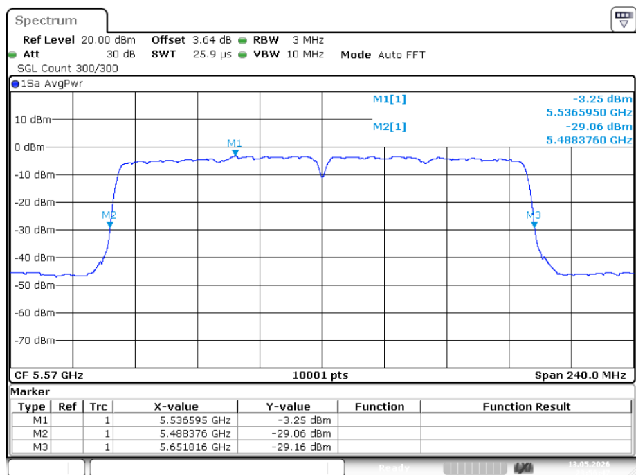
-26dB Bandwidth NVNT ac160 5570MHz Ant1
