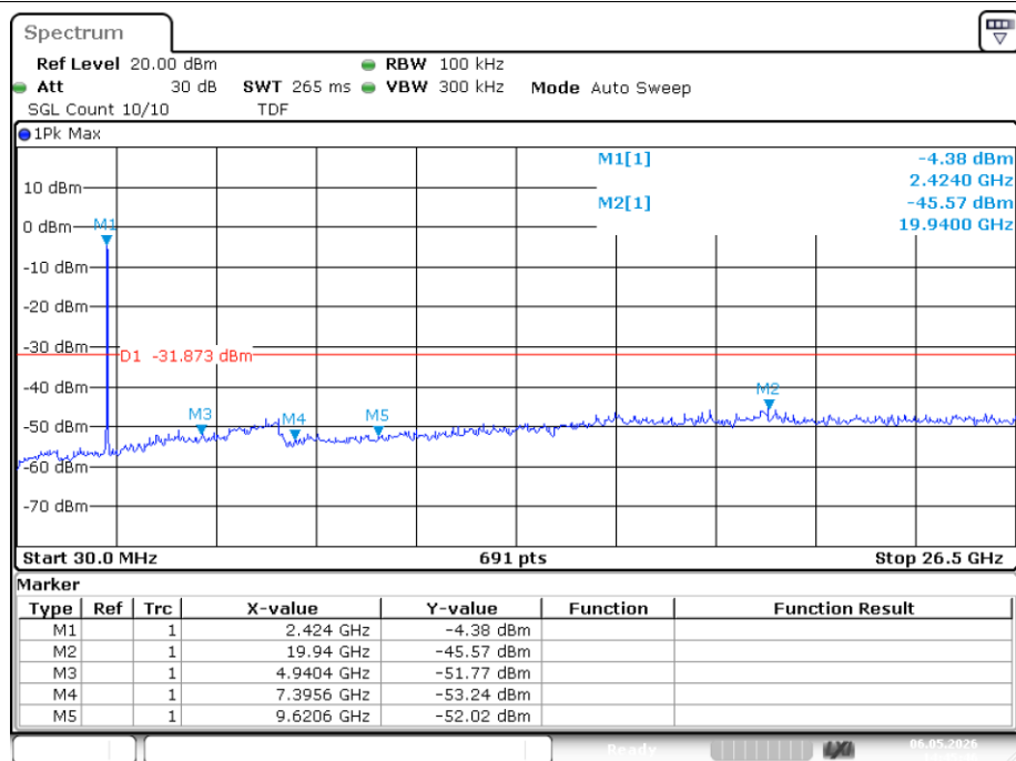
Tx. Spurious NVNT ax40 2437MHz Ant2 Ref
