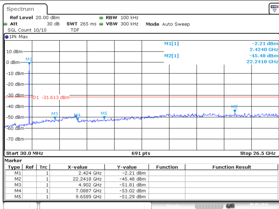
Tx. Spurious NVNT n40 2422MHz Ant2 Ref
