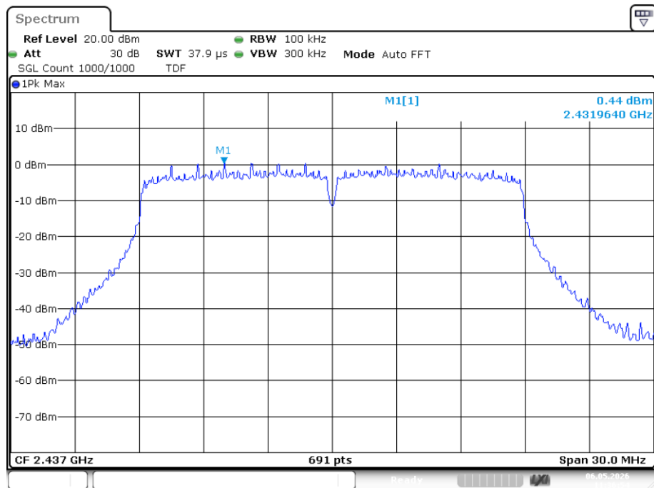
Tx. Spurious NVNT n20 2437MHz Ant2 Ref
