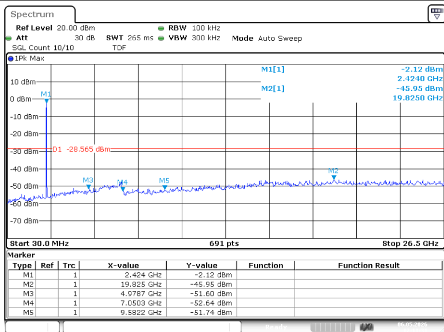
Tx. Spurious NVNT ax20 2412MHz Ant2 Ref
