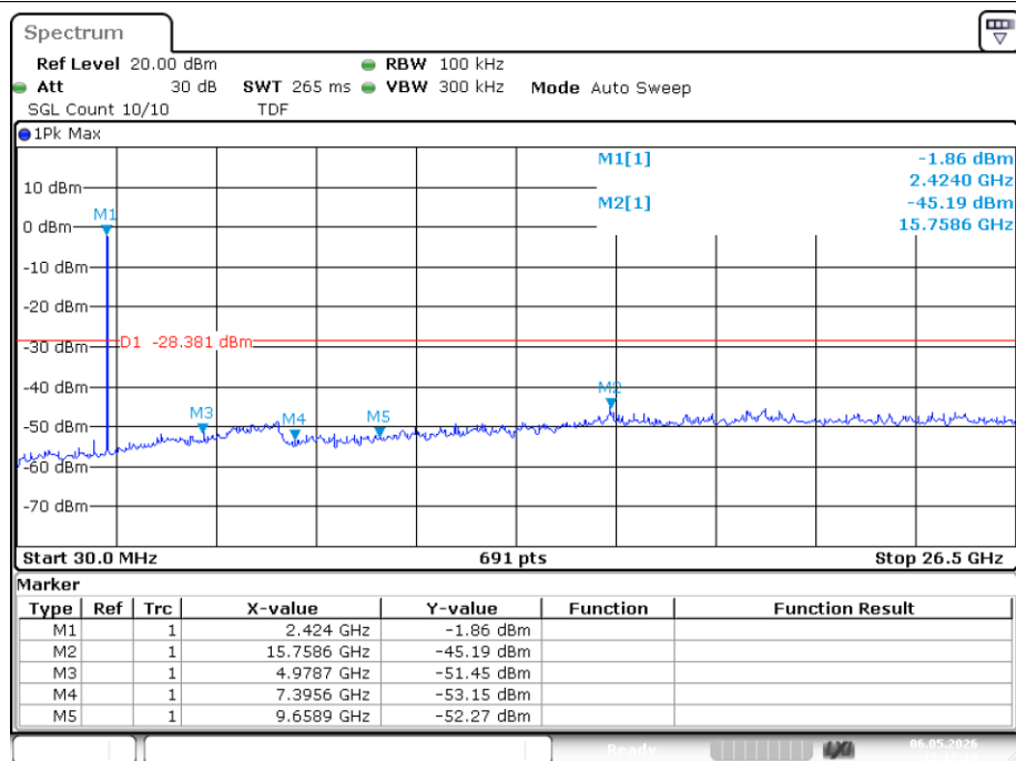
Tx. Spurious NVNT ax20 2437MHz Ant2 Ref
