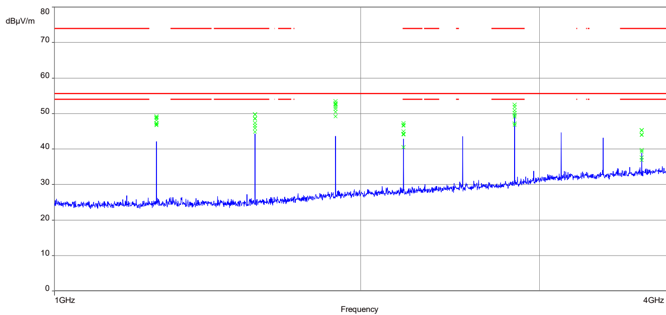
Plot 4: 1000 MHz to 4000 MHz, vertical & horizontal polarisation
