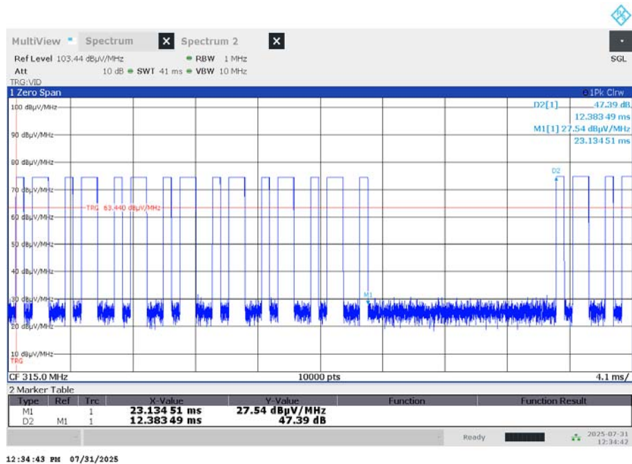
Plot 5 Silent time between two bursts: 12.4ms
