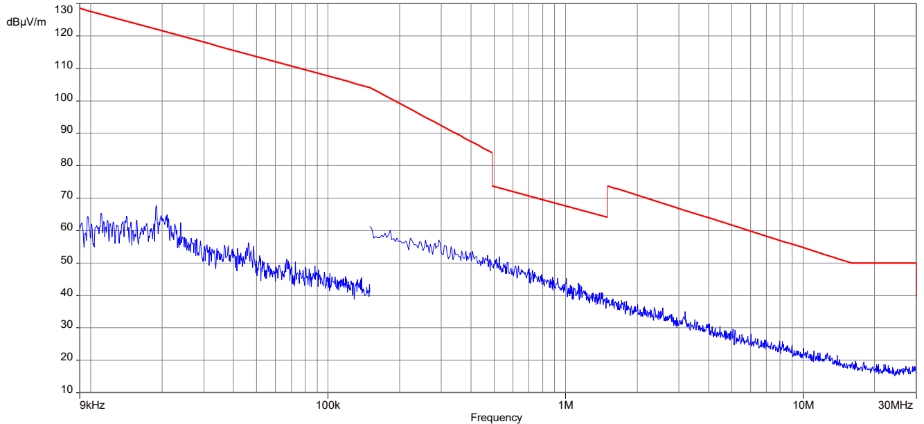
Plot 1: 9 kHz to 30 MHz, magnetic emissions FCC
