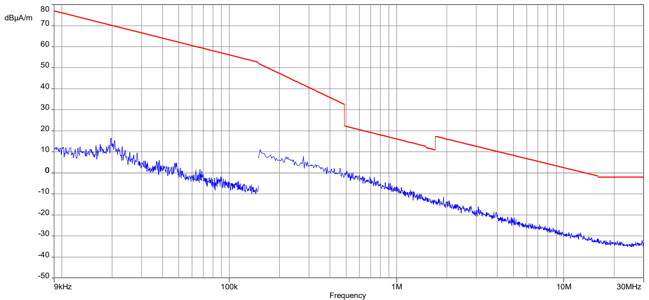
Plot 2: 9 kHz to 30 MHz, magnetic emissions IC
