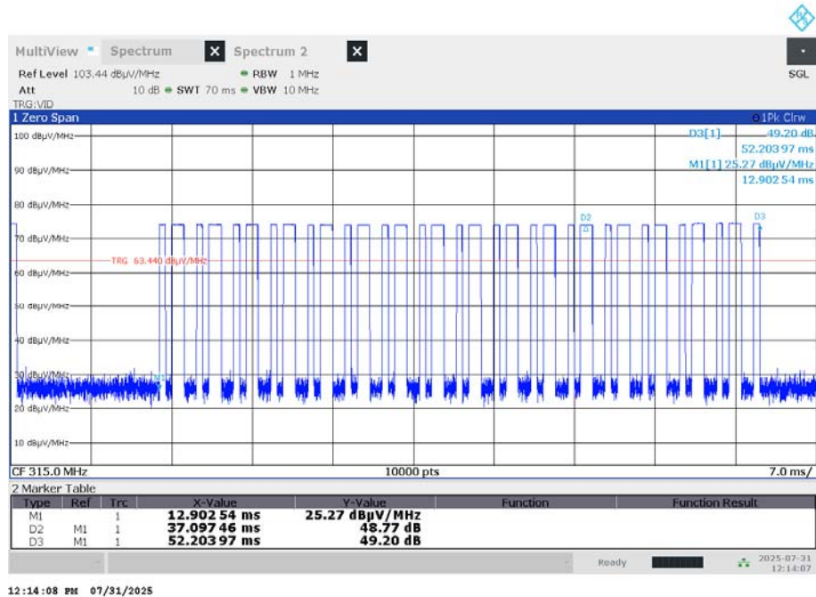
Plot 3 Burst length 52.2 ms
