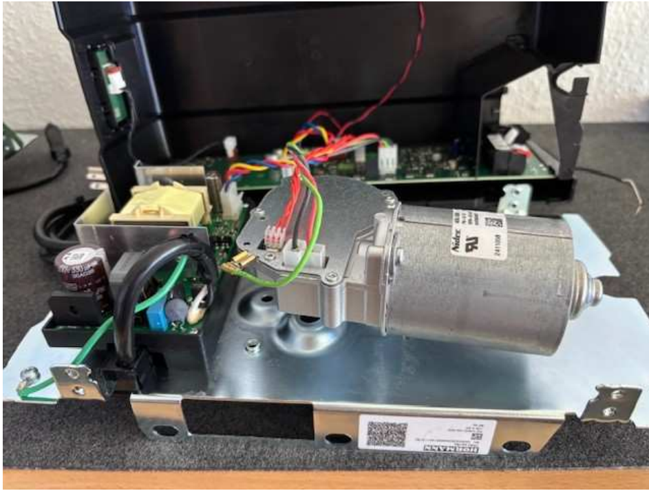
Housing opened (1)
