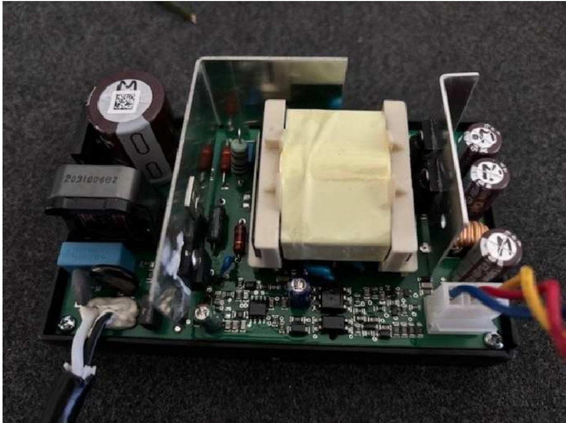
Power Supply
