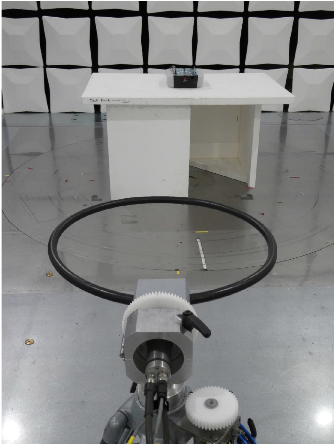
9 kHz – 30 MHz - antenna position 3
