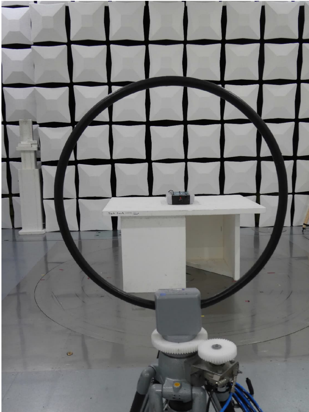
9 kHz – 30 MHz - antenna position 1
