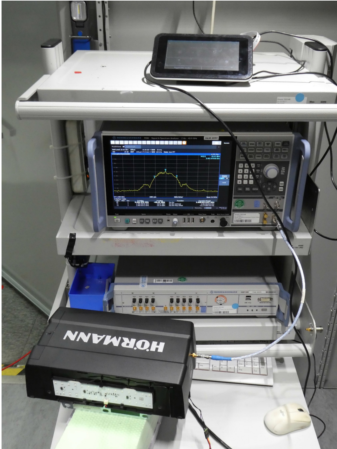
Test setup - Conducted @ antenna port
