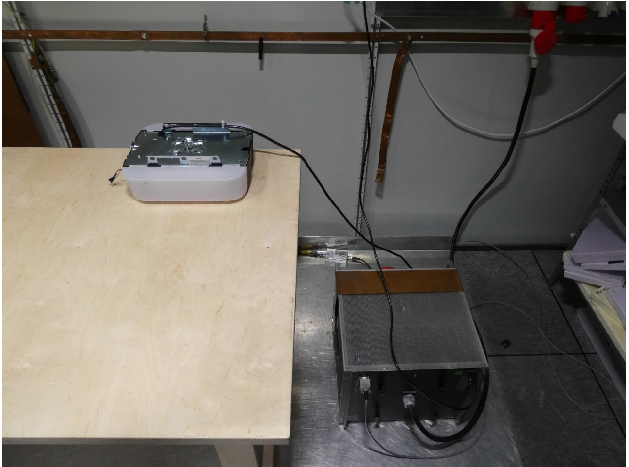
Test setup – AC power line conducted emissions
