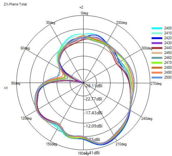
(1) X-Z Plane(unit:dBi):
