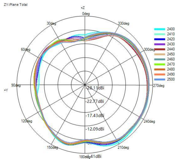
(2) Y-Z Plane(unit:dBi):
