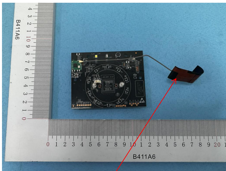
WIFI ANT
