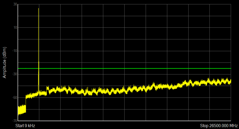
Band41 16QAM BW=15MHz Channel=40640 RB Size=1 Position=#0
