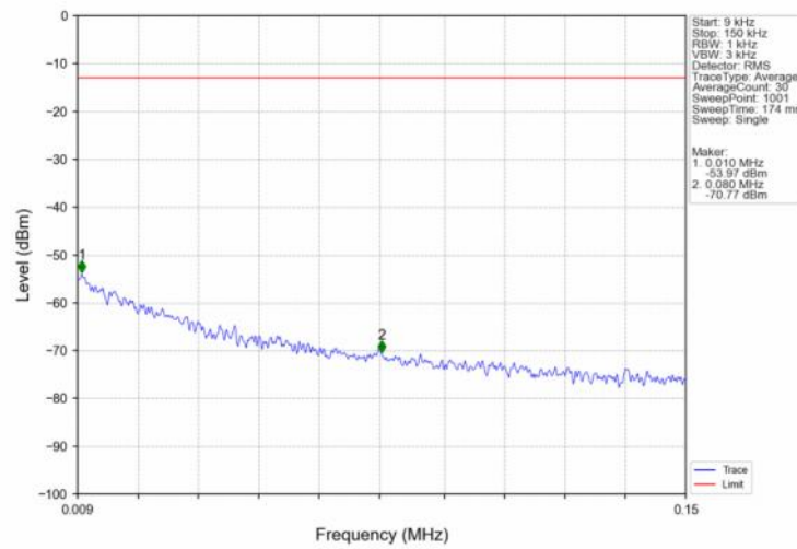
Band66_10MHz_16QAM_HCH_1775MHz_RB_1_0_NTNV
