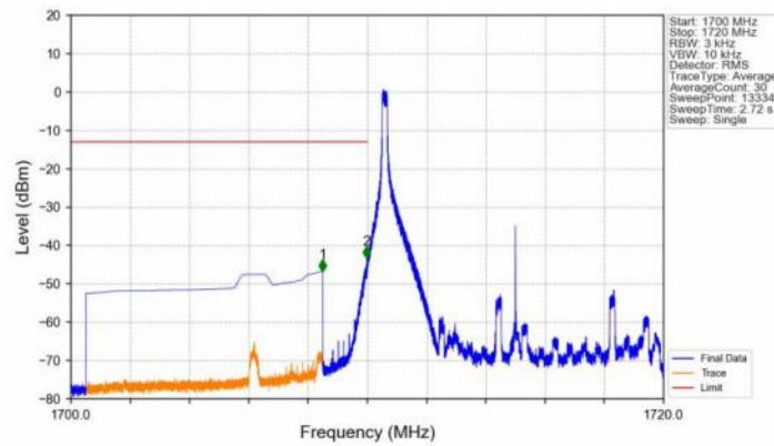
Band66_10MHz_QPSK_LCH_1715MHz_RB_1_0_NTNV
