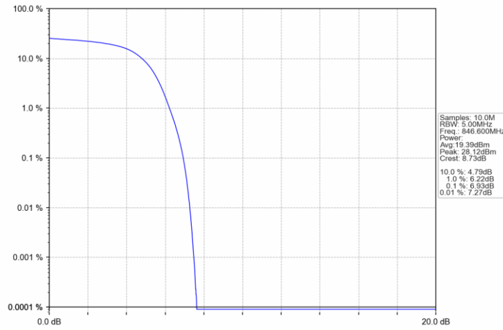
Band5_HSUPA_HCH_846.6MHz_Subtest 1_NTNV
