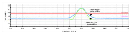
Bluetooth LE (2M) Channel 39 Peak+Average
