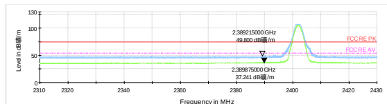
Bluetooth LE (2M) Channel 0 Peak+ Average
